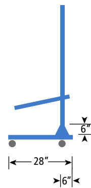
Side View: Rear-justified
