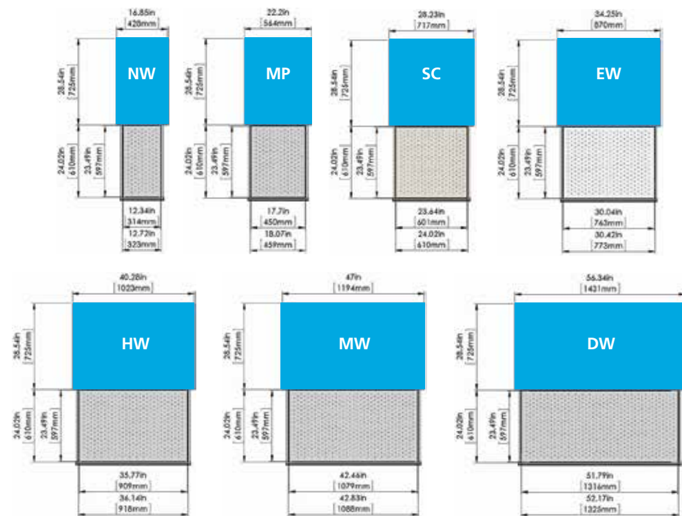
Dimensions: Full Depth Housing Footprint and Usable Drawer Space
