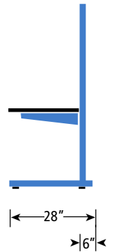
Side View: Rear-justified
