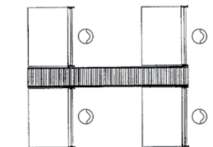
Double-Sided – operator at 90° to conveyor with standard worksurface
